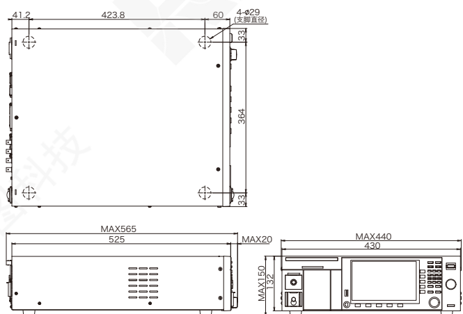
TOS9301PD
