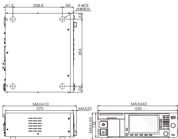
TOS9300 TOS9301
