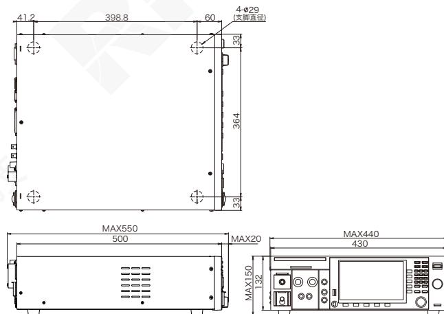
TOS9303LC
